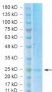
SDS-PAGE (4-20%): in vitro expressed and purified HBsAg adr protein
