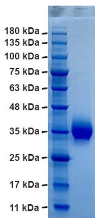
SDS-PAGE: purified recombinant spike RBD (N501Y) protein of SARS-CoV-2 UK variant
