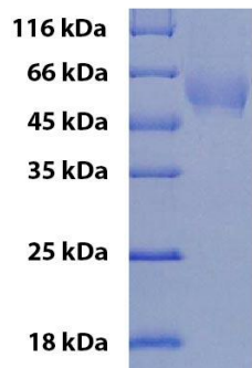
SDS-PAGE: purified HA1 (H3N2)(A/Texas/50/2012) protein.
