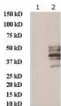
1: 293 cell extract control 2: 293 cell expressing gp41 (HXBc2)
