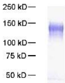
SDS-PAGE: Purified HIV-1 gp120 (pREJO4541) (Clade B) protein
