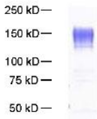
SDS-PAGE: Purified HIV-1 gp120 (pRHPA4259) (Clade B) protein
