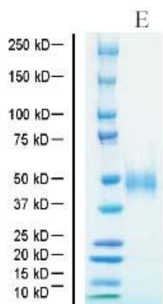
SDS-PAGE: purified HA1(H7N7) (A/Chicken/Netherlands/1/03) protein
