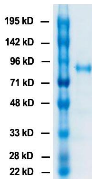
SDS-PAGE: trimerized HA (A/England/42/72)(H3N2) protein (reducing condition).
